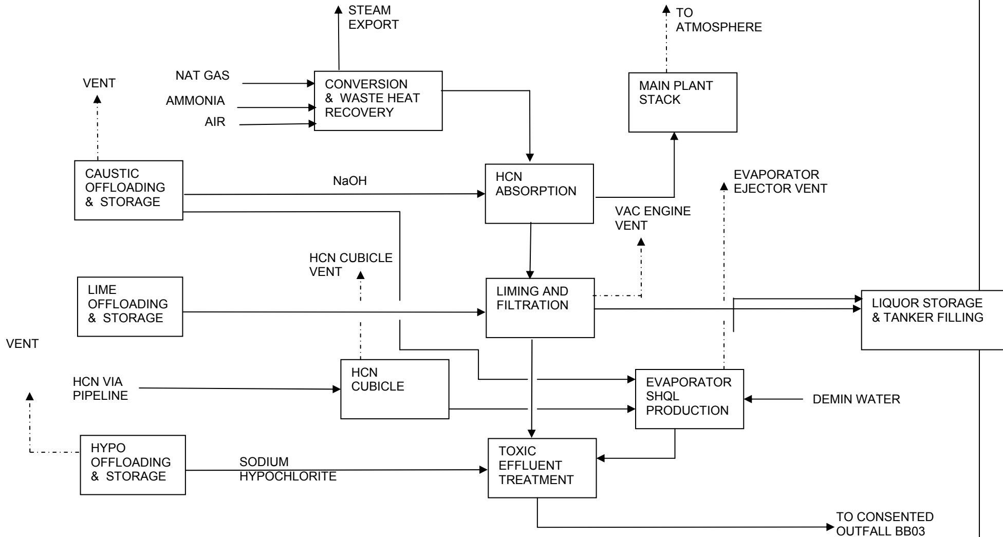
fig 2.3.1 NaCN Plant: Process Flow Diagram
